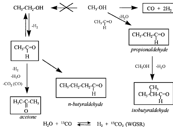
FIG. 11. Reaction scheme for methanol-acetaldehyde reactions on \text{K-CuMg}_5\text{CeO}_x catalysts.
