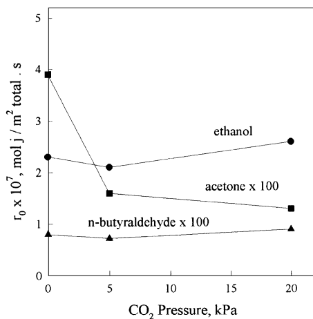
FIG. 9. CO 2 effect on ethanol reactions. Rates of ethanol consumption and of product formation as a function of CO 2 initial pressure on 1.0 wt.% K-Cu 0.5 Mg 5 CeO x . [573 K, 101.3 kPa total pressure, 4.0 kPa ethanol, 26.7 kPa dihydrogen, balance He.]
